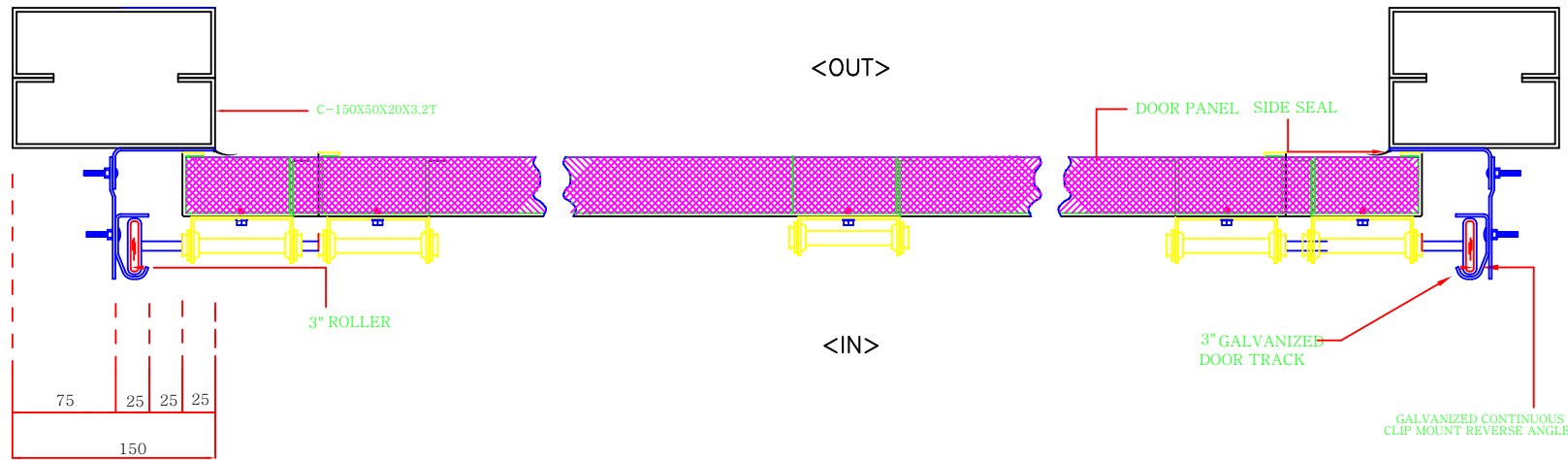
1 JAMB DETAIL (PLAN) SCALE 1/10
