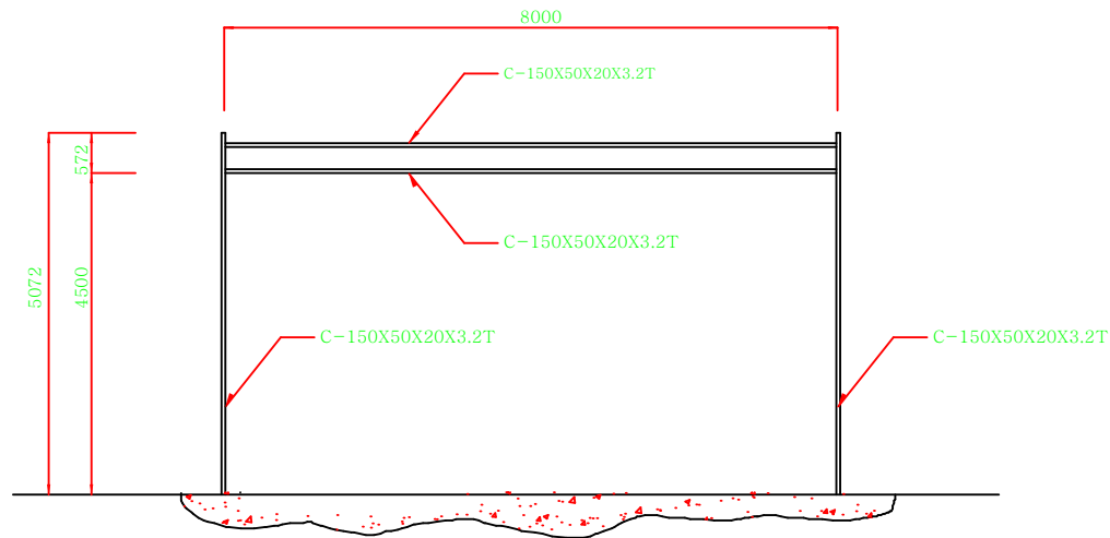
2 FRAME ELEVATION SCALE 1/100
