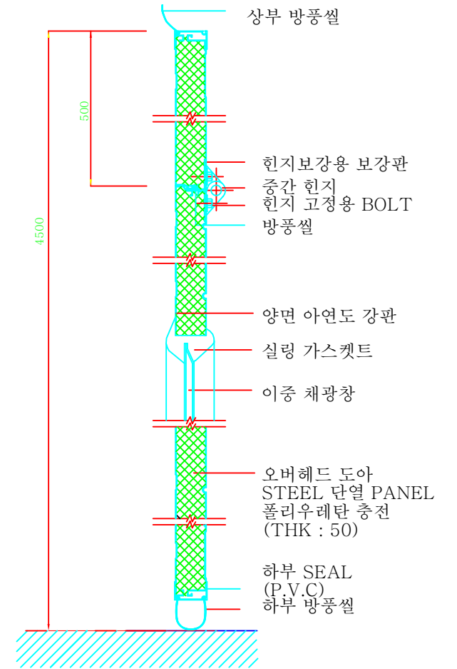
3 SECTION CONSTRUCTION NONE SCALE
